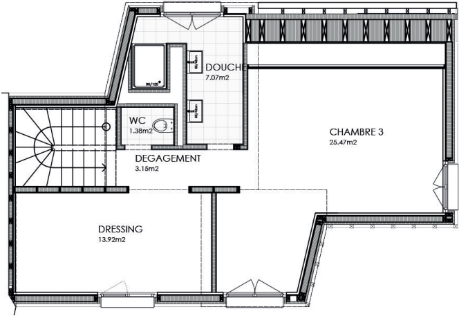
Combles
